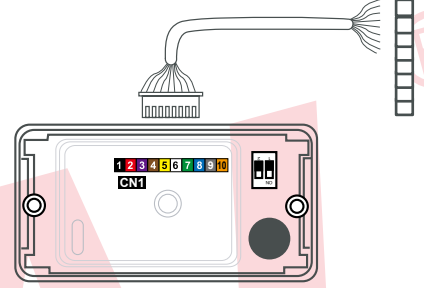
WG34 AR-721U [13.56MHz]
